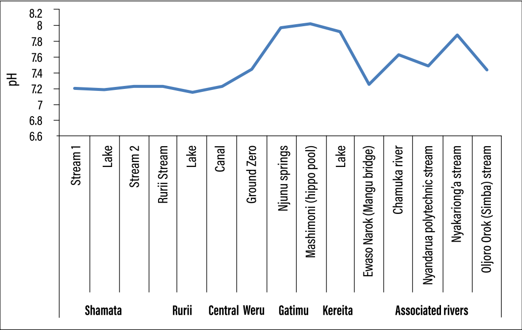
Figure 22: Water pH levels across the sampling sites
